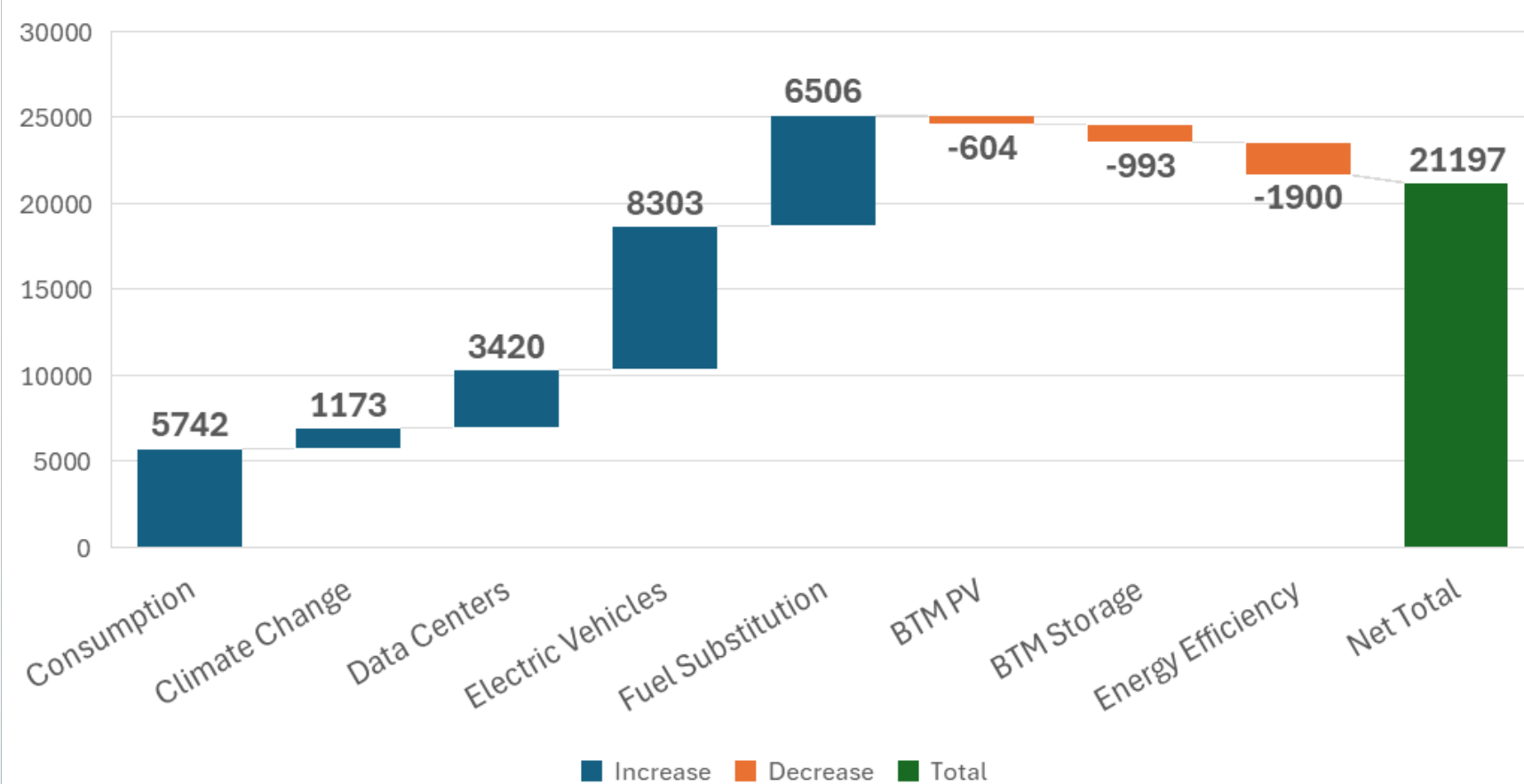
CED 2024 Planning - CAISO load growth (MW) from 2024 to 2040 (September, hour ending 18)
